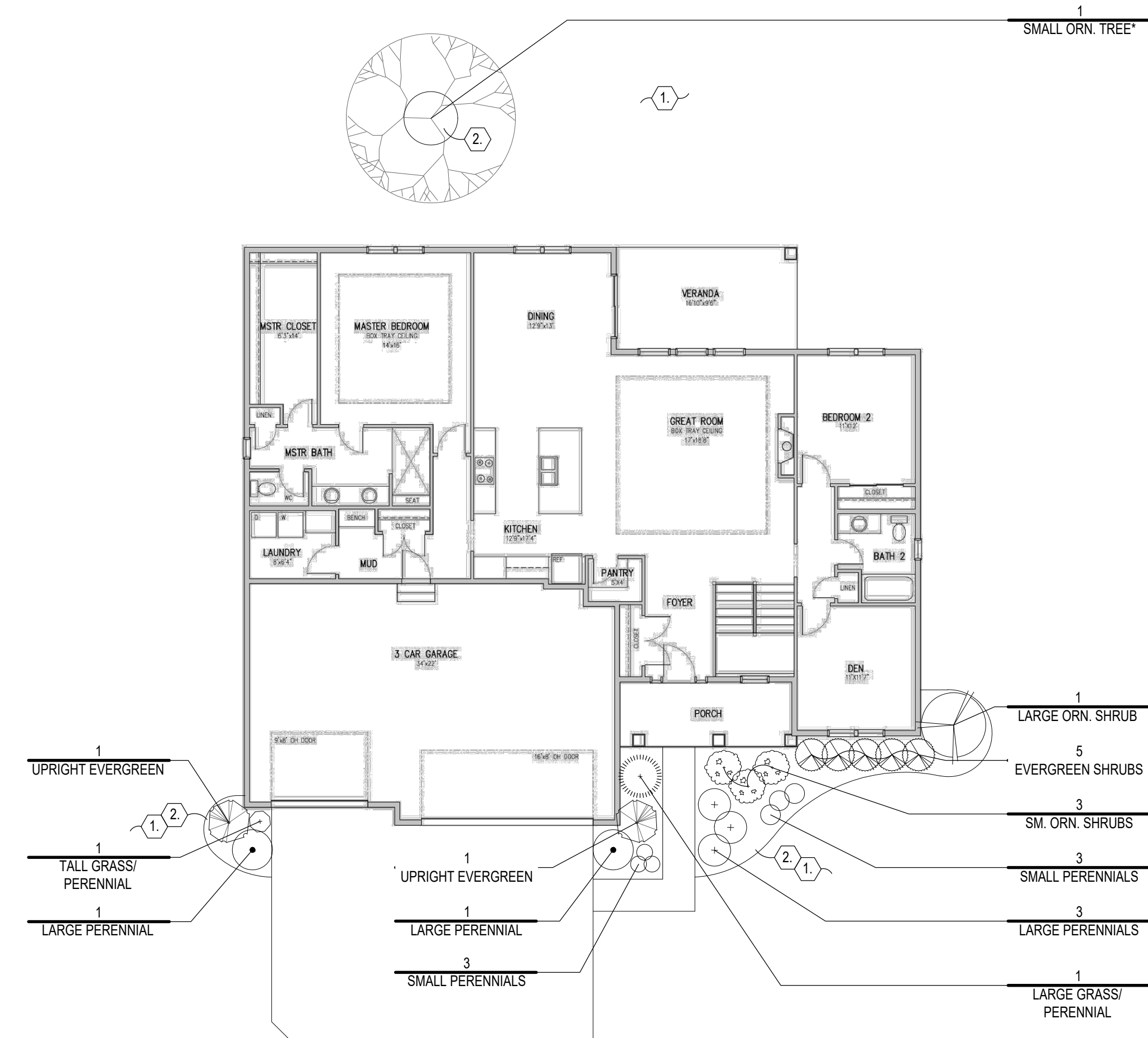
BUILDING TYPICAL LANDSCAPE PLAN (REFER TO PLANT LISTS A&B)
