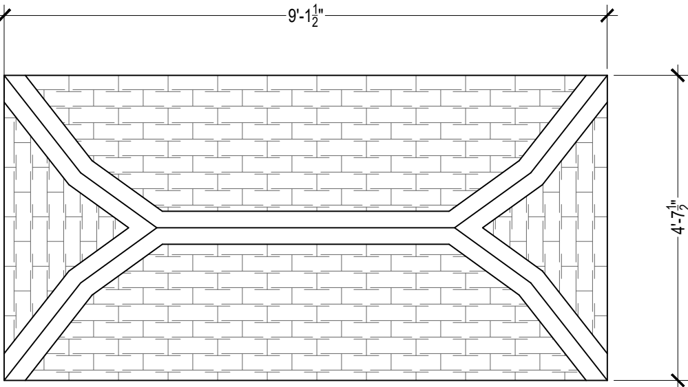
PLAN VIEW - ROOF
