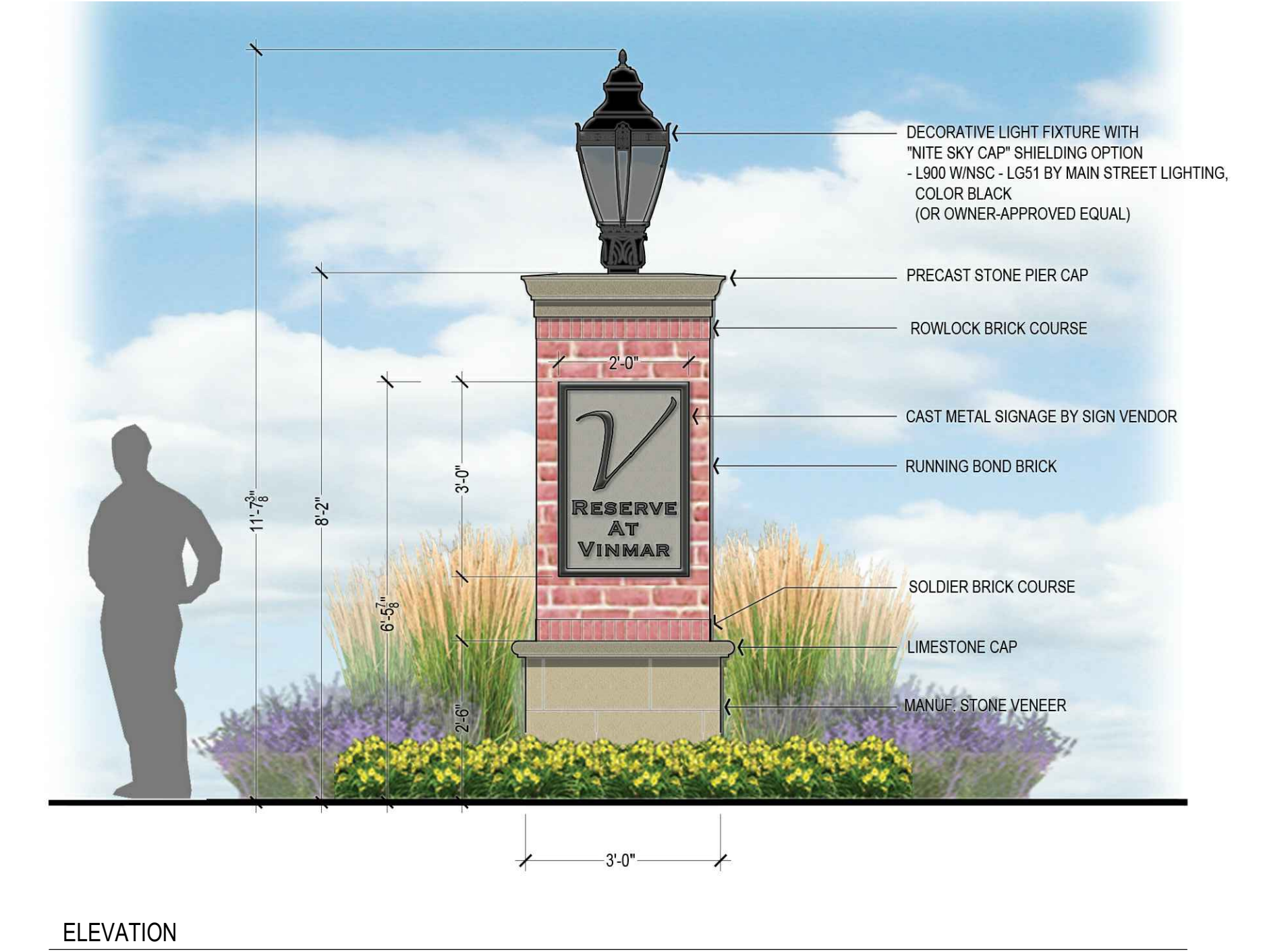
ENTRY COLUMN (FINAL COLOR SELECTIONS BY OWNER) SCALE: 1/2" = 1'-0"
