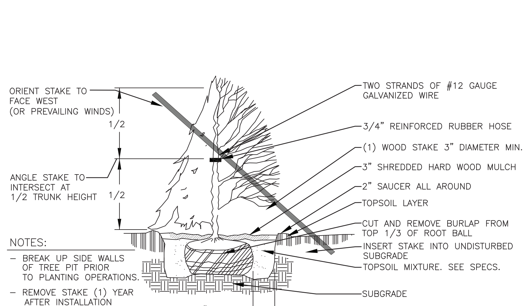
2 Evergreen Planting Detail
