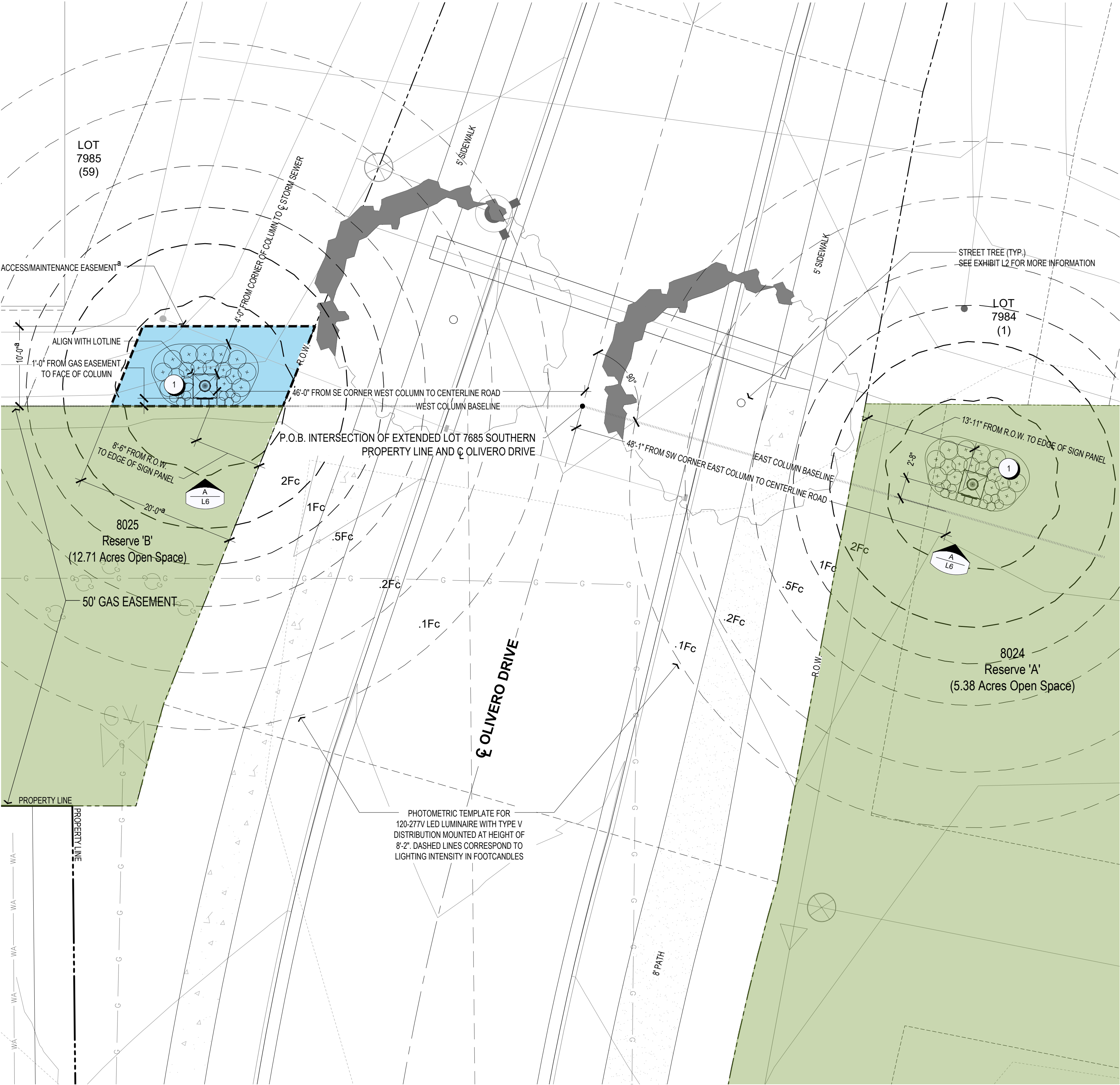
ENTRY COLUMNS - LAYOUT AND MATERIALS PLAN
