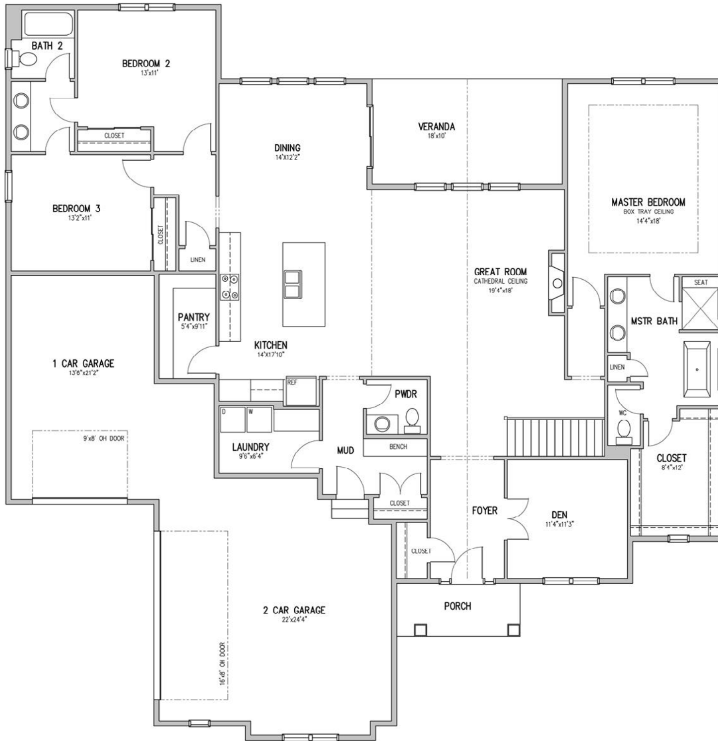
PLAN A - 2515 SF
