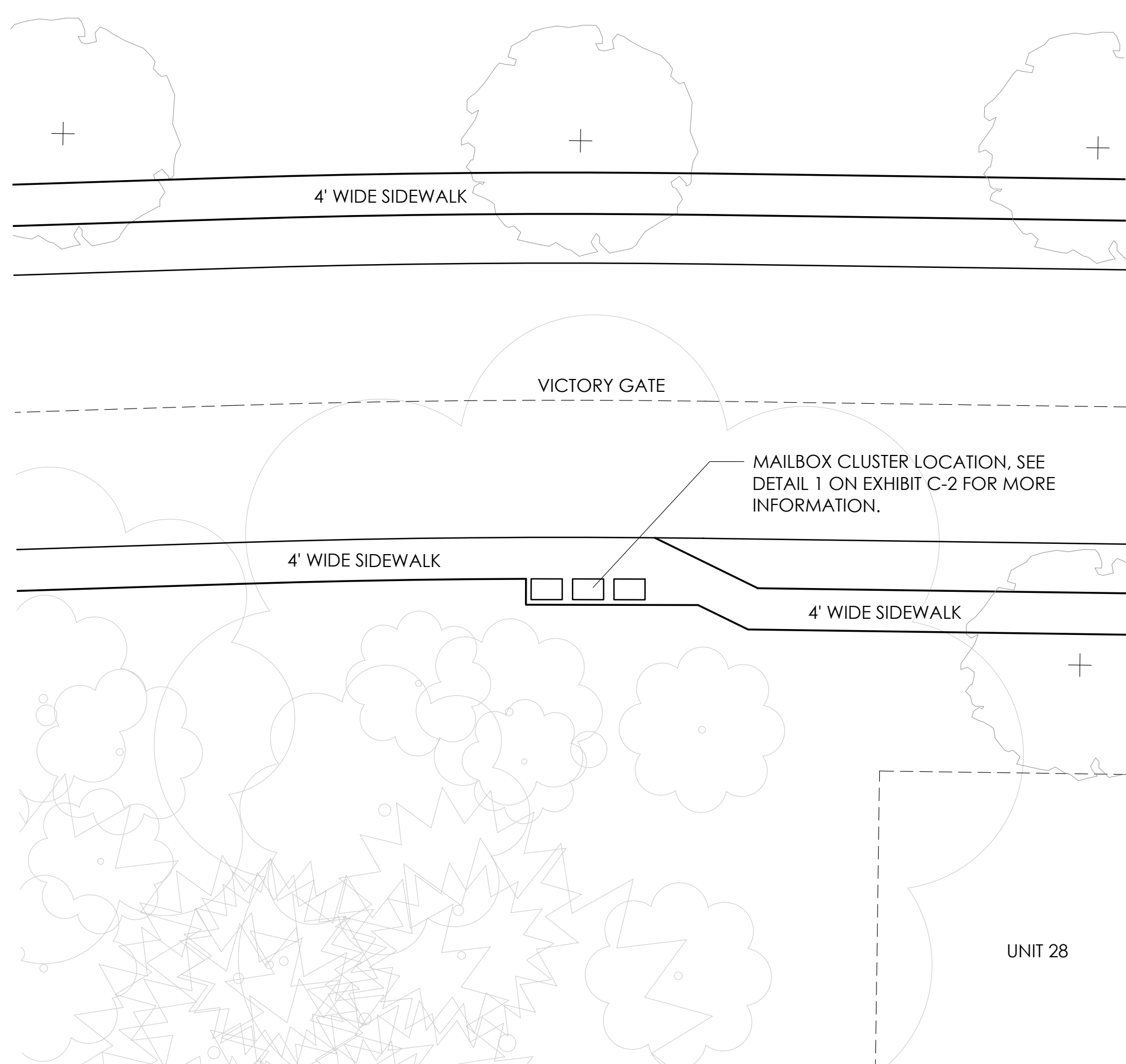
2 MAILBOX LOCATION ENLARGEMENT PLAN SCALE: 1" = 10'
