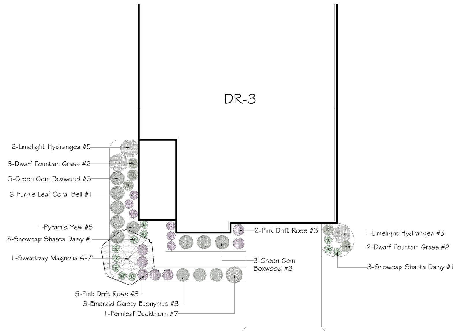
④ VERONA (DR-3) TYPICAL FRONT LANDSCAPE PLAN SCALE: N.T.S.
