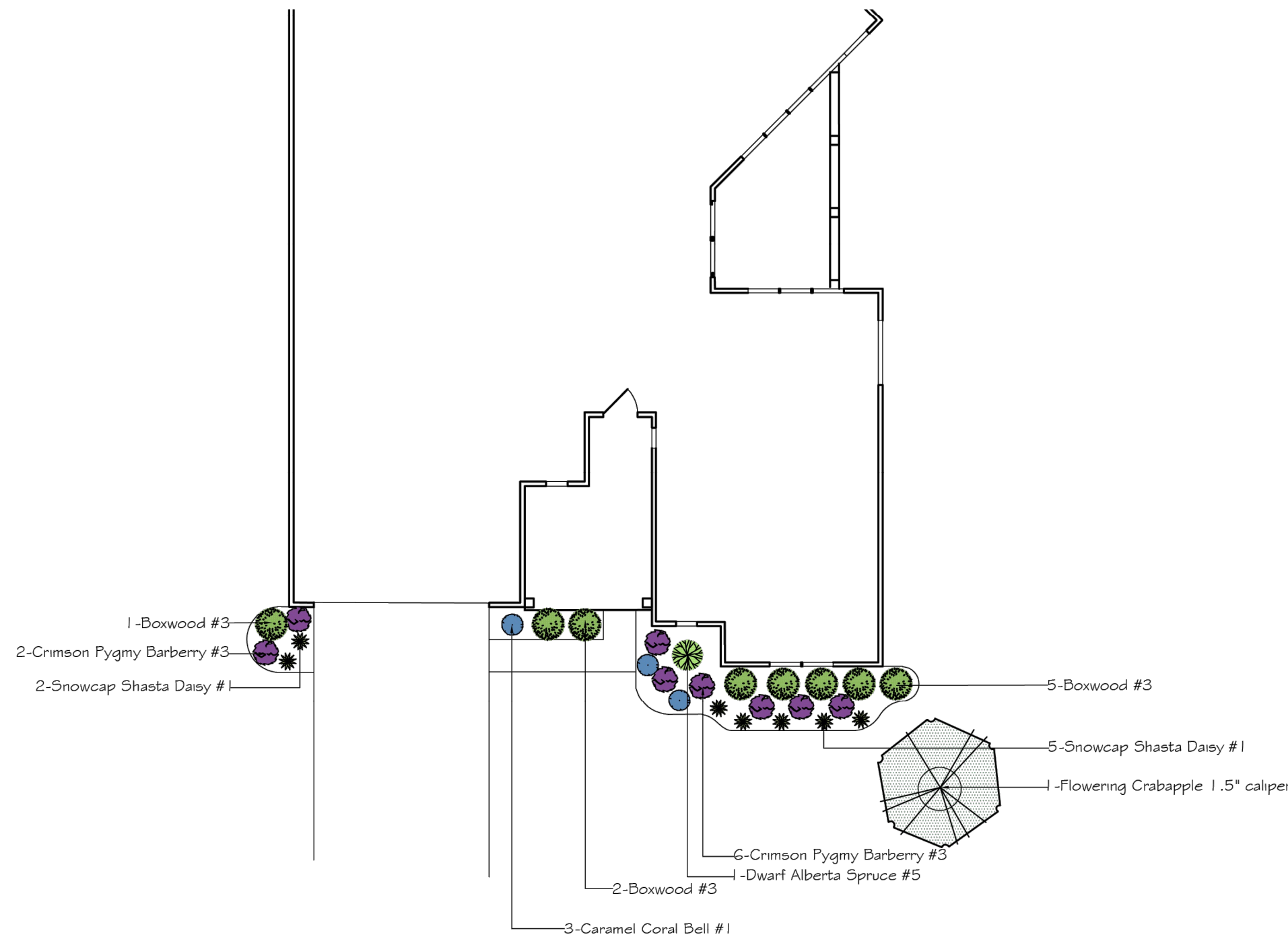
⑧ PROVENANCE (EL-1) TYPICAL FRONT LANDSCAPE PLAN SCALE: N.T.S.
