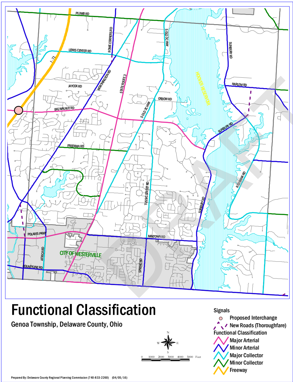
FIGURE 3.18 – FUNCTIONAL CLASSIFICATION OF ROADWAYS AND PROPOSED ROADS
