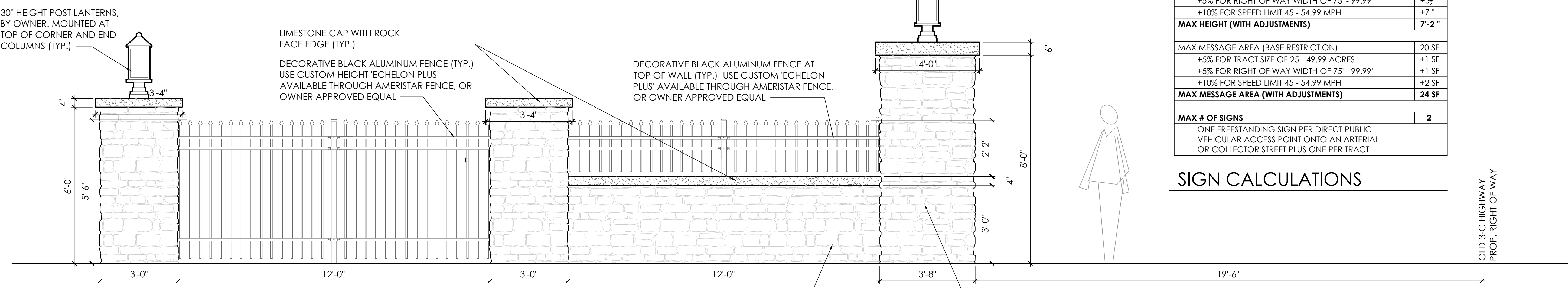
3 ENTRY FEATURE ELEVATION - INTERNAL 'ROAD A' (BOTH SIDES) SCALE 1/2" = 1'
