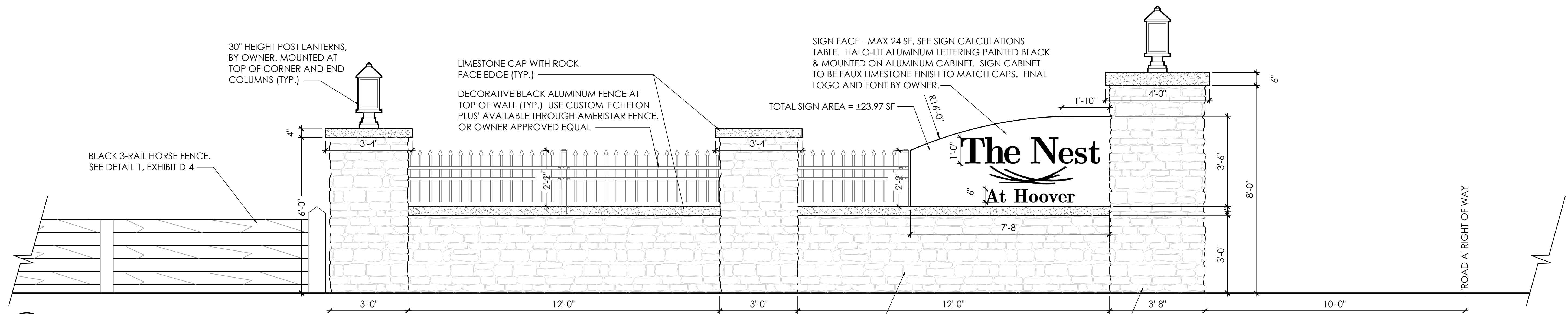
1 ENTRY FEATURE/SIGN ELEVATION - OLD 3C HIGHWAY NORTH SCALE 1/2" = 1'
